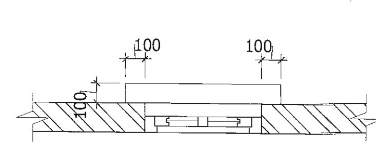
TYPICAL VENTILATOR CHAJJA DETAILS
