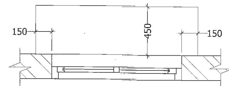
TYPICAL WINDOW CHAJJA DETAILS
